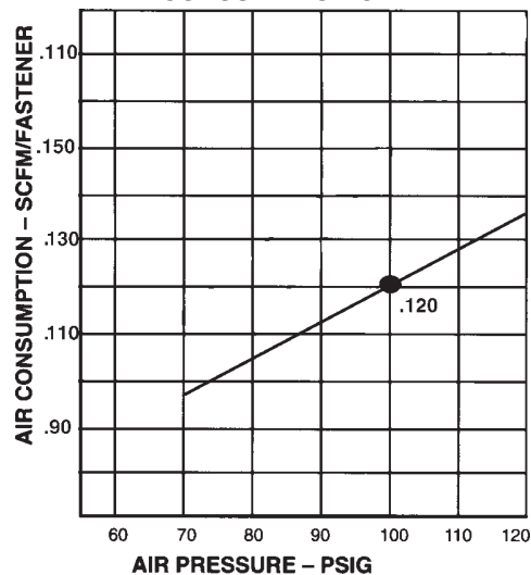
AIR CONSUMPTION CHART
